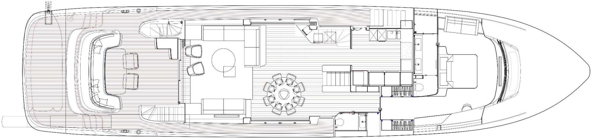
MAIN DECK
